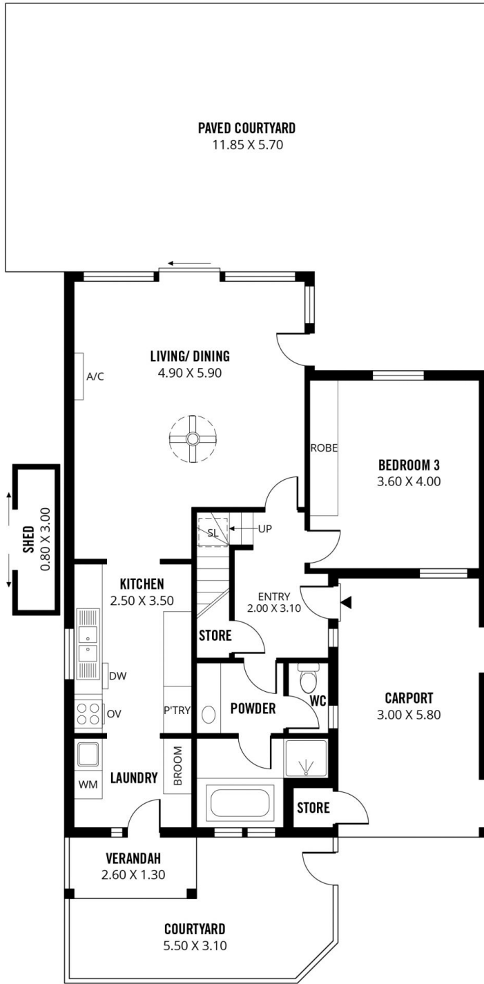
GROUND FLOOR
