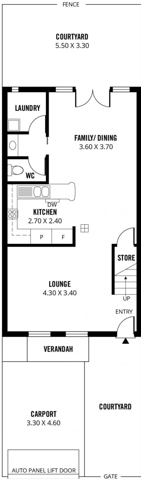
GROUND FLOOR
