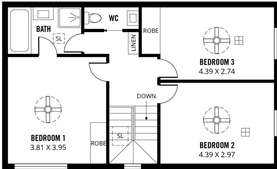
UPPER FLOOR
