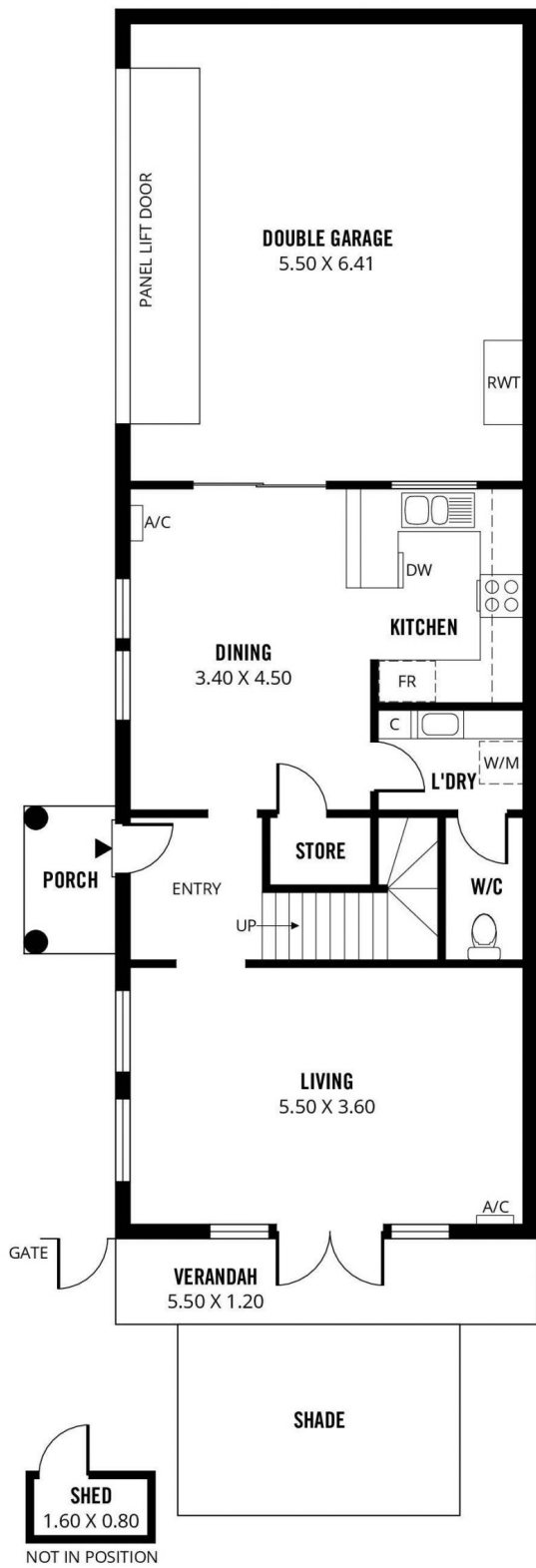
GROUND FLOOR
