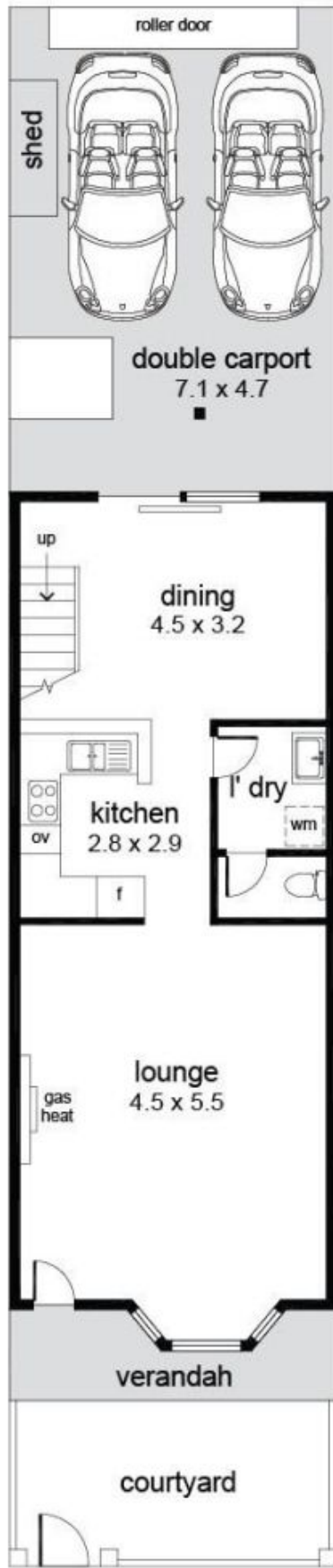
ground floor
